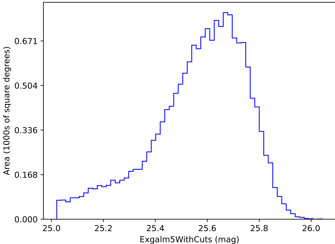
weather_cloudso36v3.4_10yrs i band non-DD year 2: ExgalM5WithCuts
