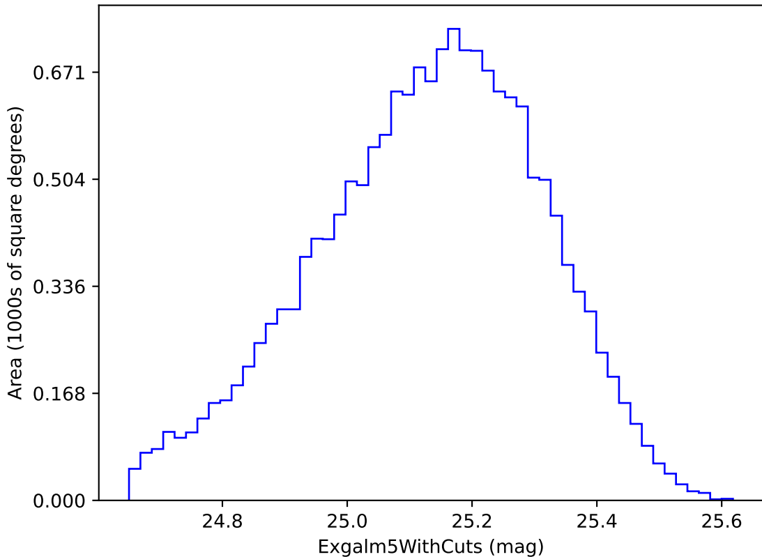
weather_cloudso36v3.4_10yrs i band non-DD year 1: Exgalml5WithCuts
