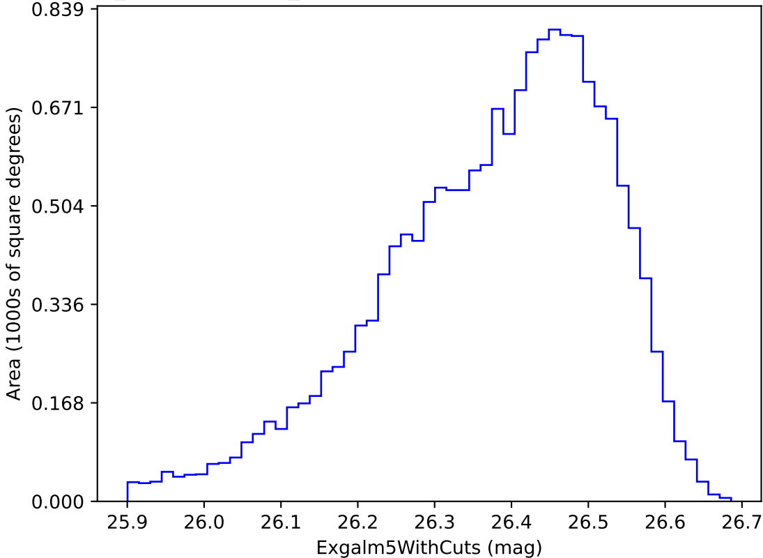
weather_cloudso36v3.4_10yrs i band non-DD year 10: Exgalml5WithCuts
