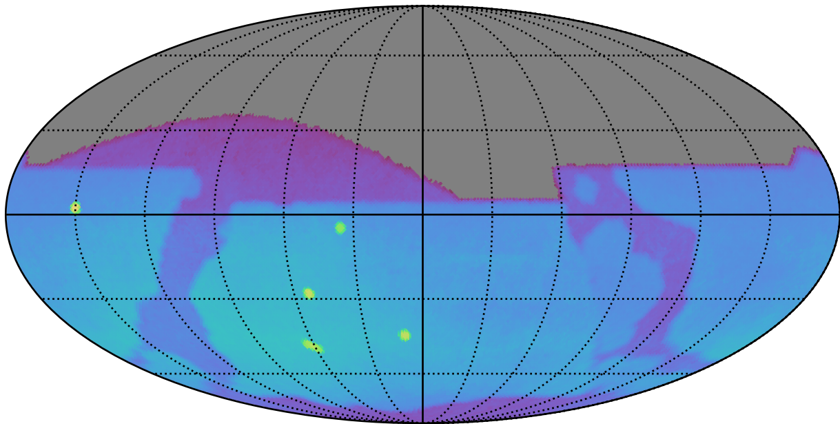
weather_cloudso36v3.4_10yrs : Brown Dwarf, L7
