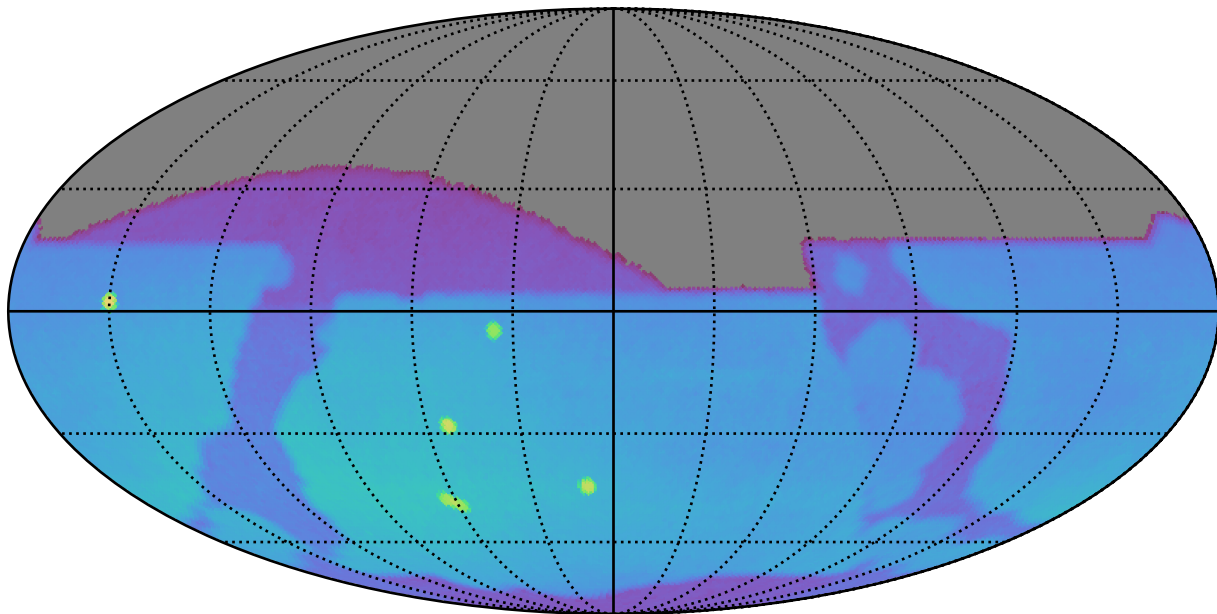
weather_cloudso36v3.4_10yrs : Brown Dwarf, L4
