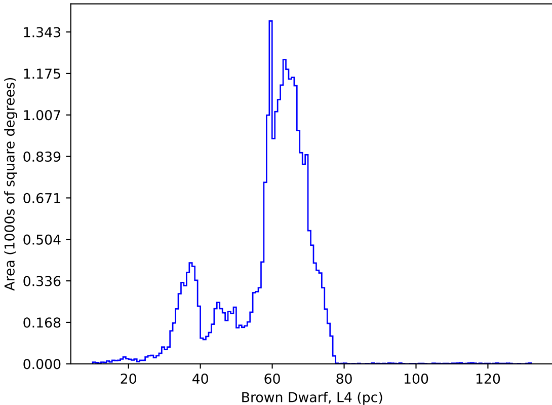
weather_cloudso36v3.4_10yrs : Brown Dwarf, L4
