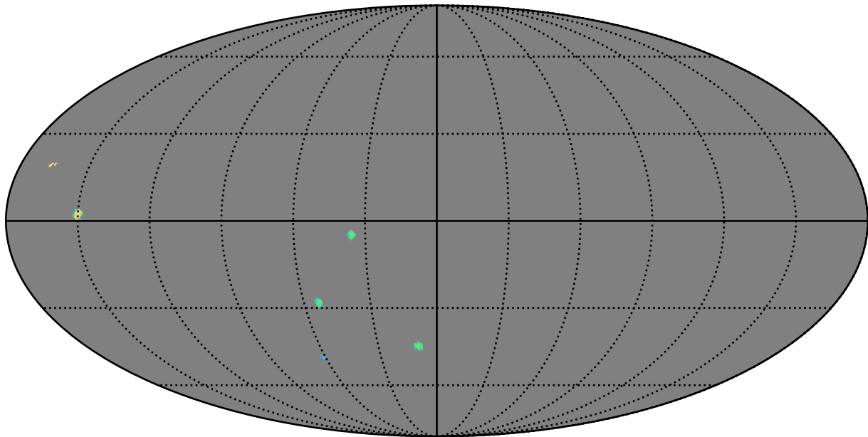
weather_cloudso36v3.4_10yrs z band: AGN_TimeLag_5_days
