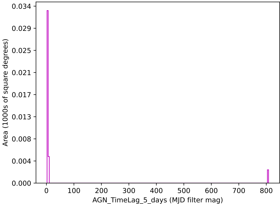
weather_cloudso36v3.4_10yrs z band: AGN_TimeLag_5_days
