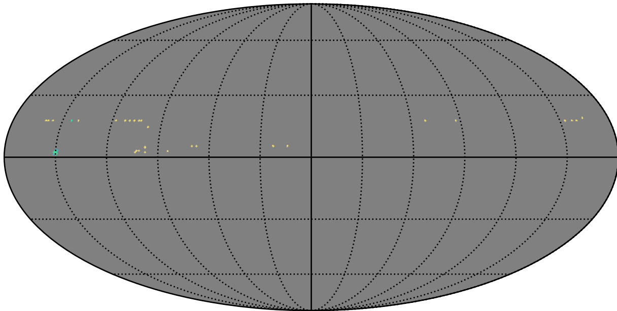
weather_cloudso36v3.4_10yrs y band: AGN_TimeLag_5_days
