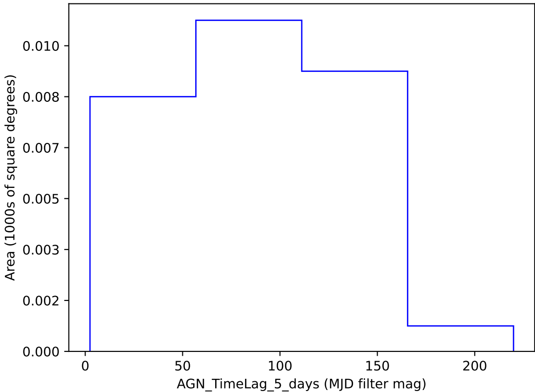
weather_cloudso36v3.4_10yrs y band: AGN_TimeLag_5_days
