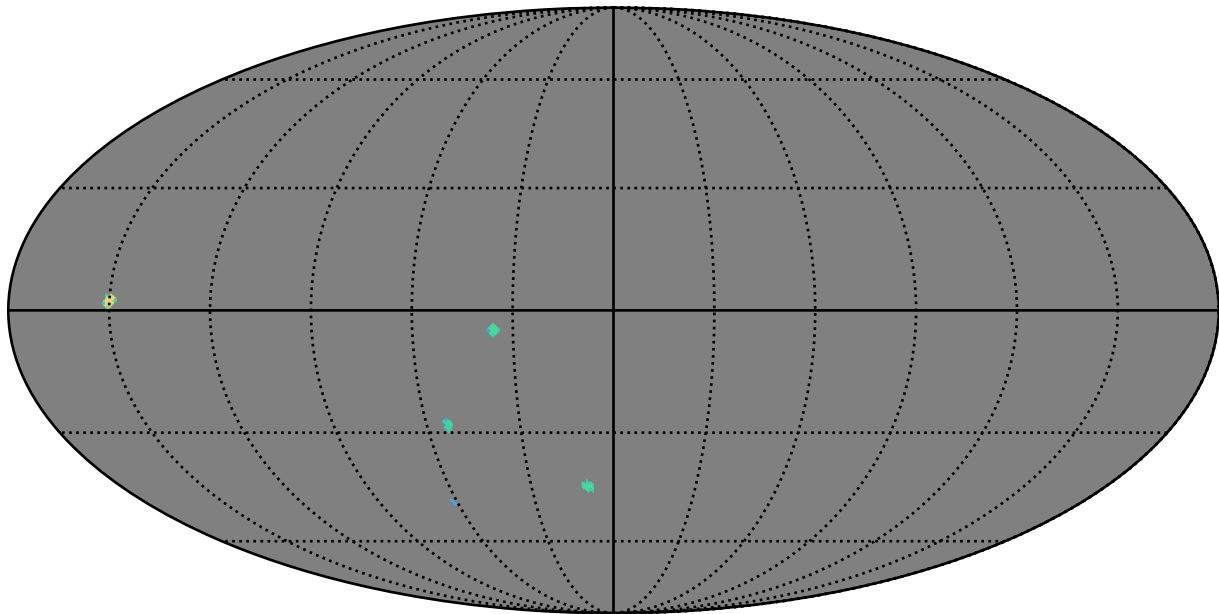
weather_cloudso36v3.4_10yrs r band: AGN_TimeLag_5_days
