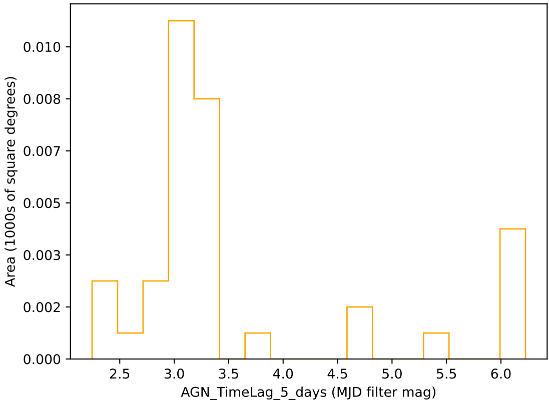
weather_cloudso36v3.4_10yrs r band: AGN_TimeLag_5_days
