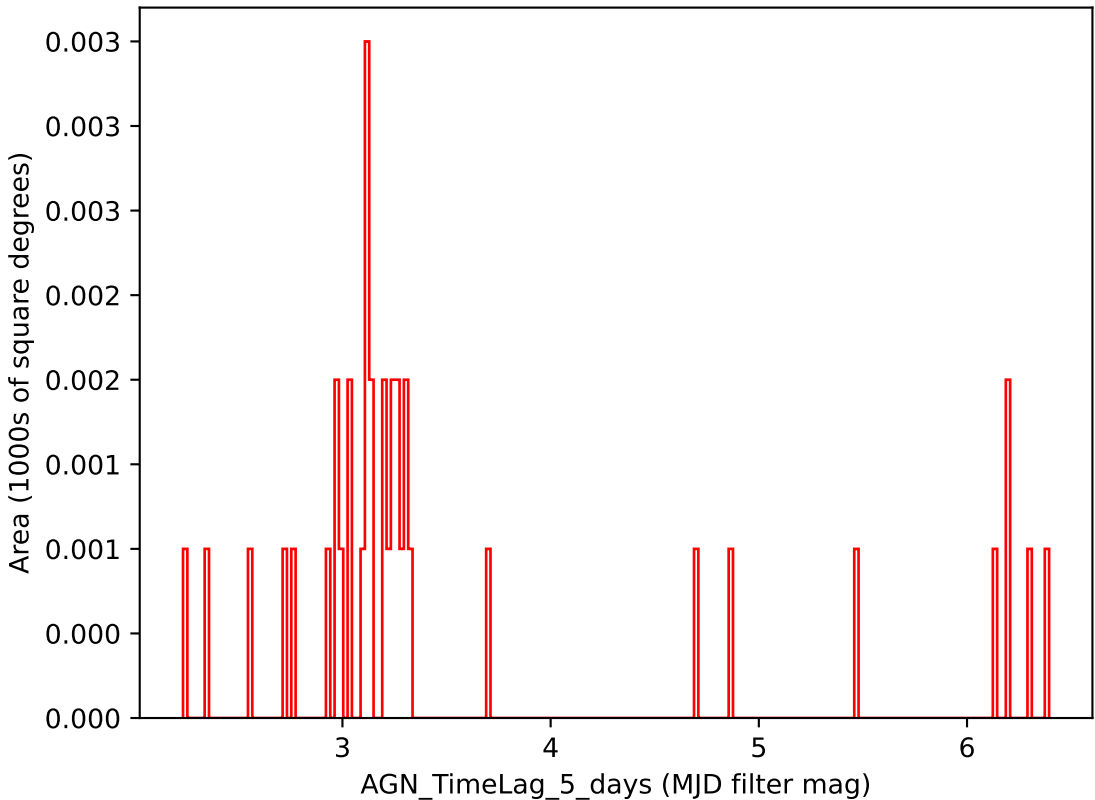
weather_cloudso36v3.4_10yrs i band: AGN_TimeLag_5_days
