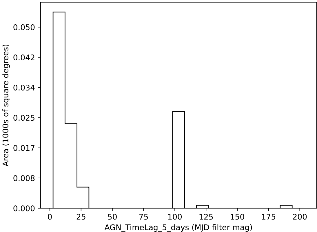
weather_cloudso36v3.4_10yrs all bands: AGN_TimeLag_5_days
