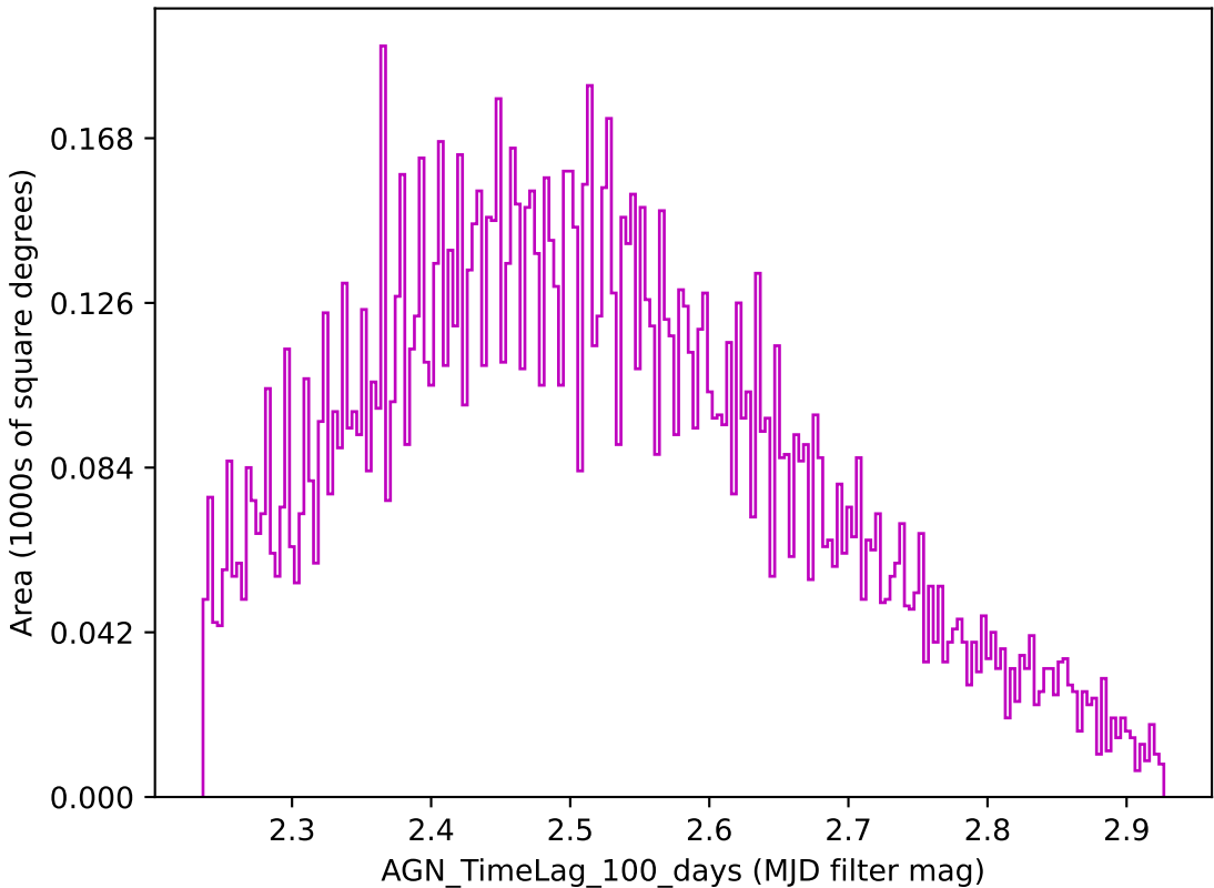
weather_cloudso36v3.4_10yrs z band: AGN_TimeLag_100_days
