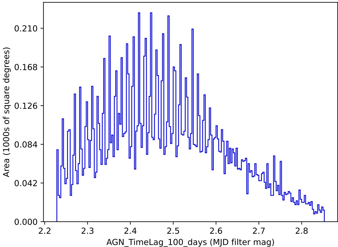
weather_cloudso36v3.4_10yrs y band: AGN_TimeLag_100_days
