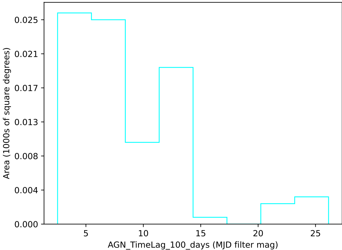
weather_cloudso36v3.4_10yrs u band: AGN_TimeLag_100_days
