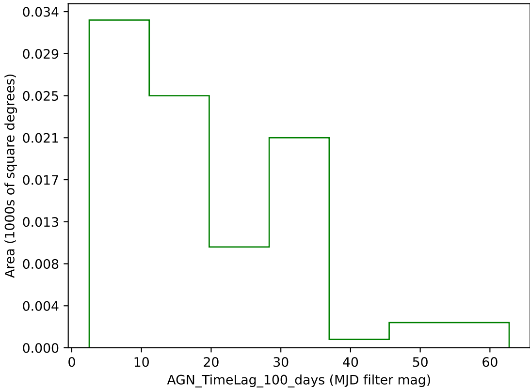
weather_cloudso36v3.4_10yrs g band: AGN_TimeLag_100_days
