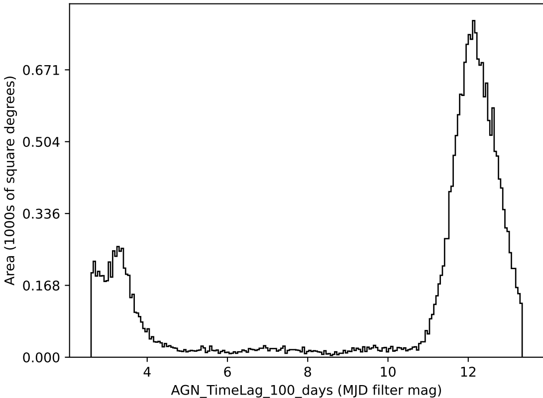
weather_cloudso36v3.4_10yrs all bands: AGN_TimeLag_100_days
