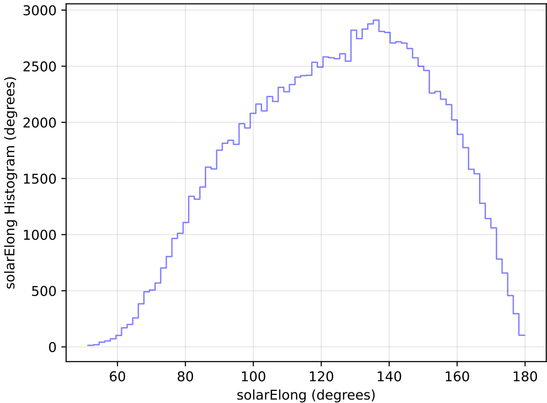
weather_cloudso36v3.4_10yrs WFD u band: solarElong Histogram
