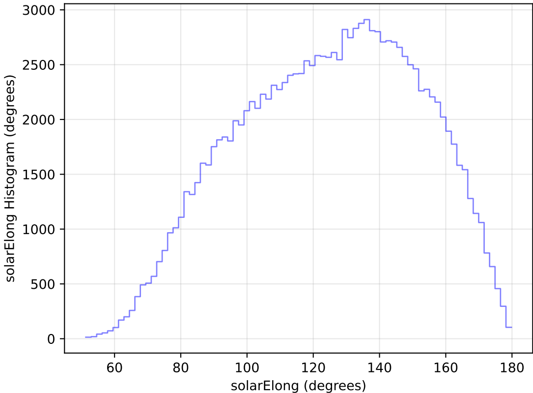
weather_cloudso36v3.4_10yrs All sky u band: solarElong Histogram
