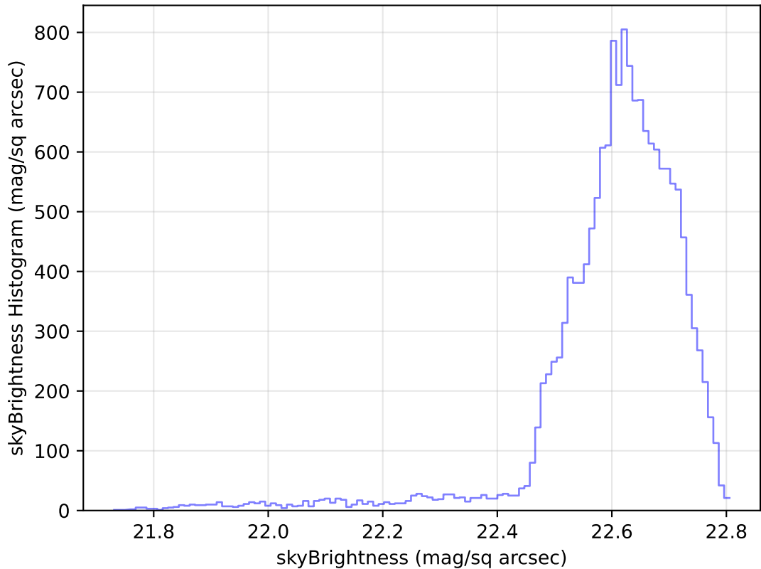
weather_cloudso36v3.4_10yrs Yr 1 u band: skyBrightness Histogram
