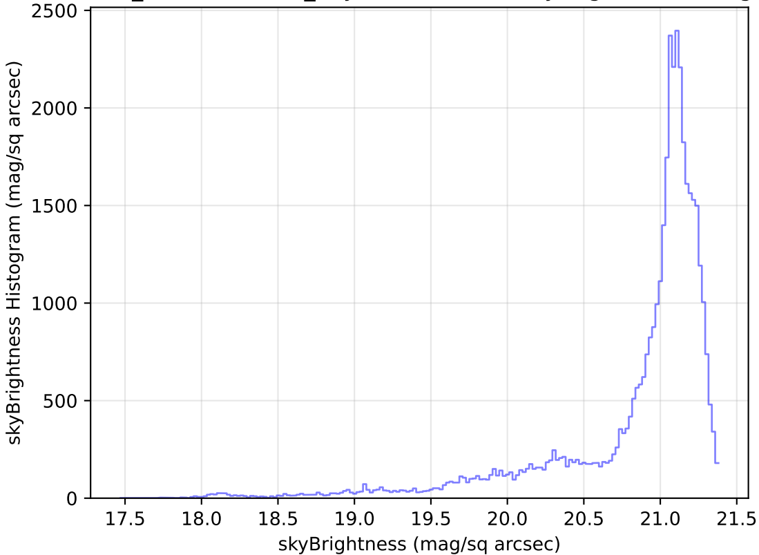
weather_cloudso36v3.4_10yrs Yr 1 r band: skyBrightness Histogram
