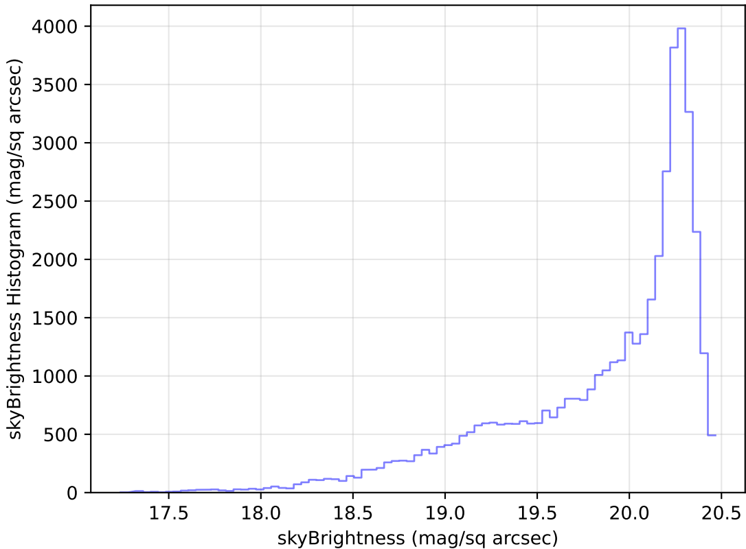
weather_cloudso36v3.4_10yrs Yr 1 i band: skyBrightness Histogram
