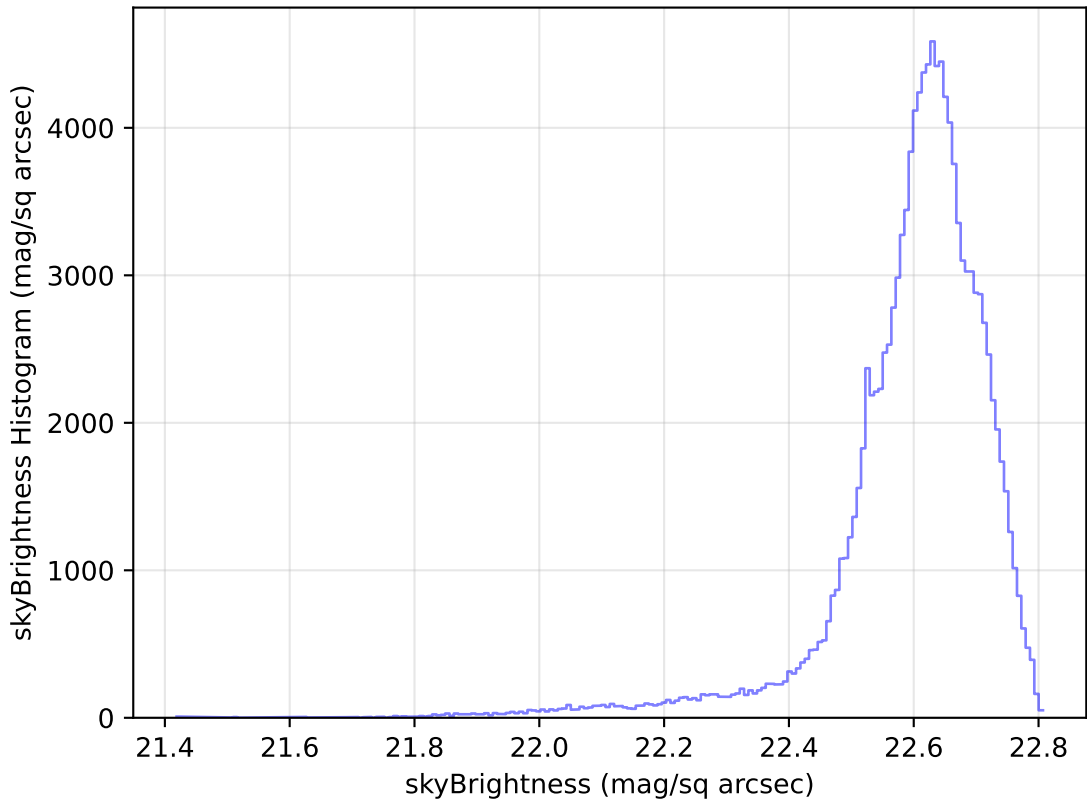
weather_cloudso36v3.4_10yrs WFD u band: skyBrightness Histogram
