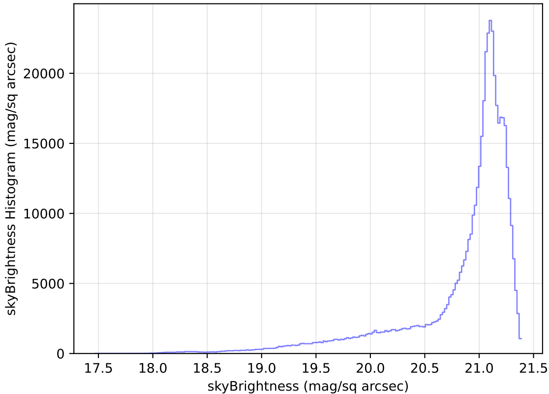
weather_cloudso36v3.4_10yrs WFD r band: skyBrightness Histogram
