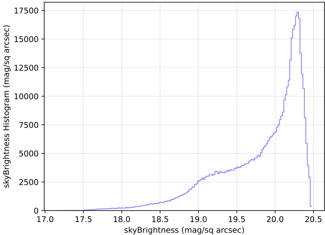
weather_cloudso36v3.4_10yrs WFD i band: skyBrightness Histogram
