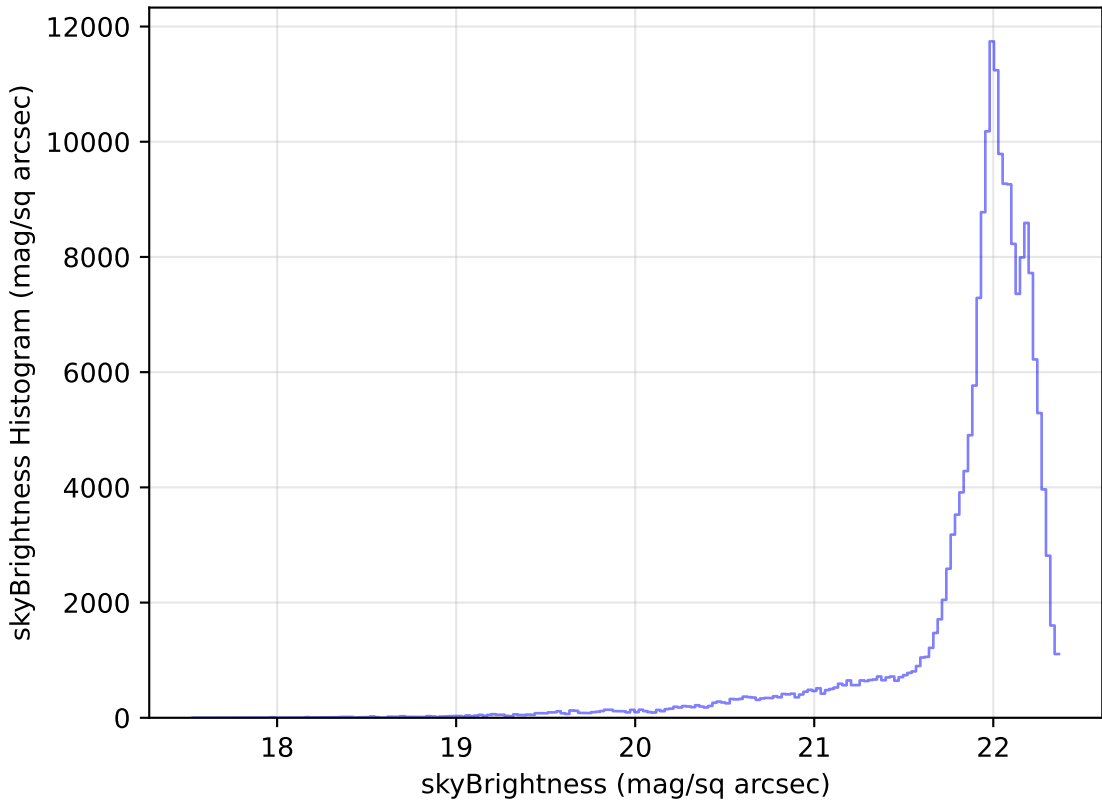
weather_cloudso36v3.4_10yrs WFD g band: skyBrightness Histogram
