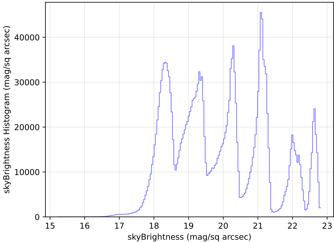
weather_cloudso36v3.4_10yrs WFD all bands: skyBrightness Histogram
