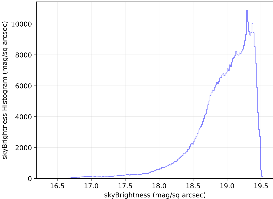
weather_cloudso36v3.4_10yrs All sky z band: skyBrightness Histogram
