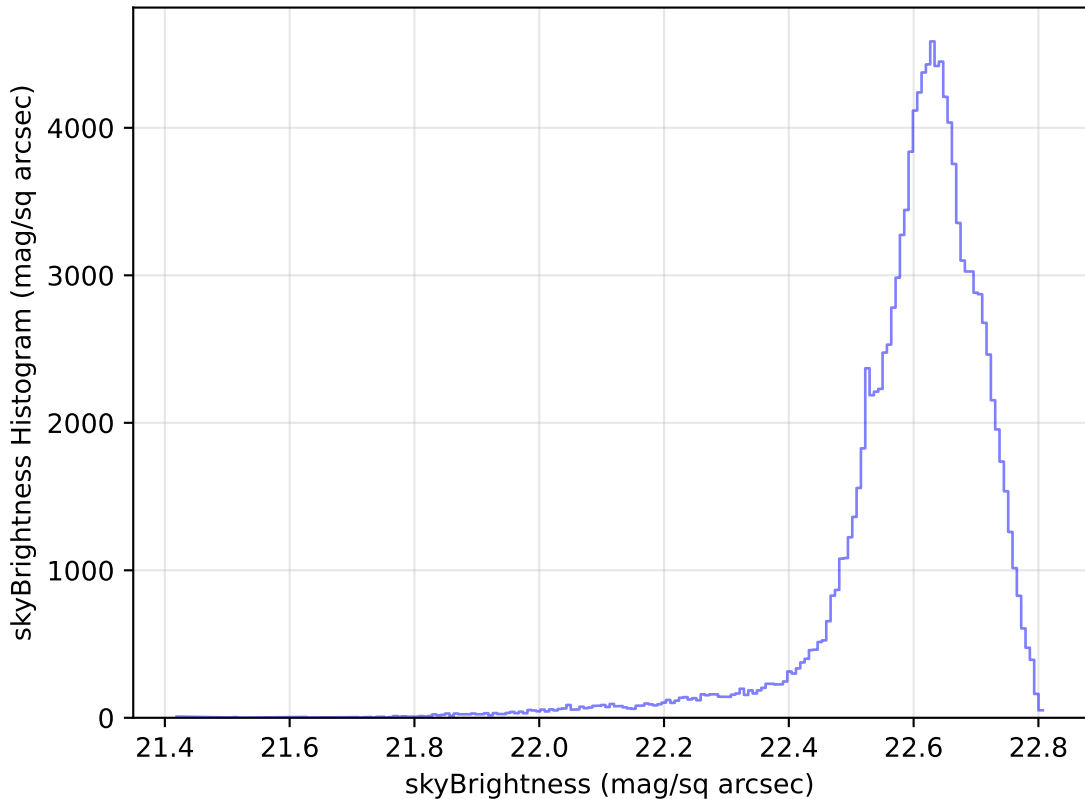
weather_cloudso36v3.4_10yrs All sky u band: skyBrightness Histogram
