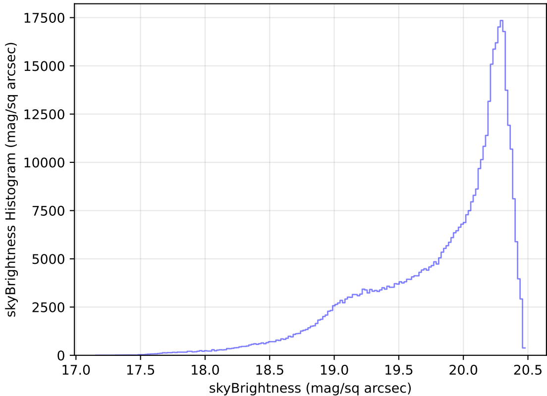
weather_cloudso36v3.4_10yrs All sky i band: skyBrightness Histogram
