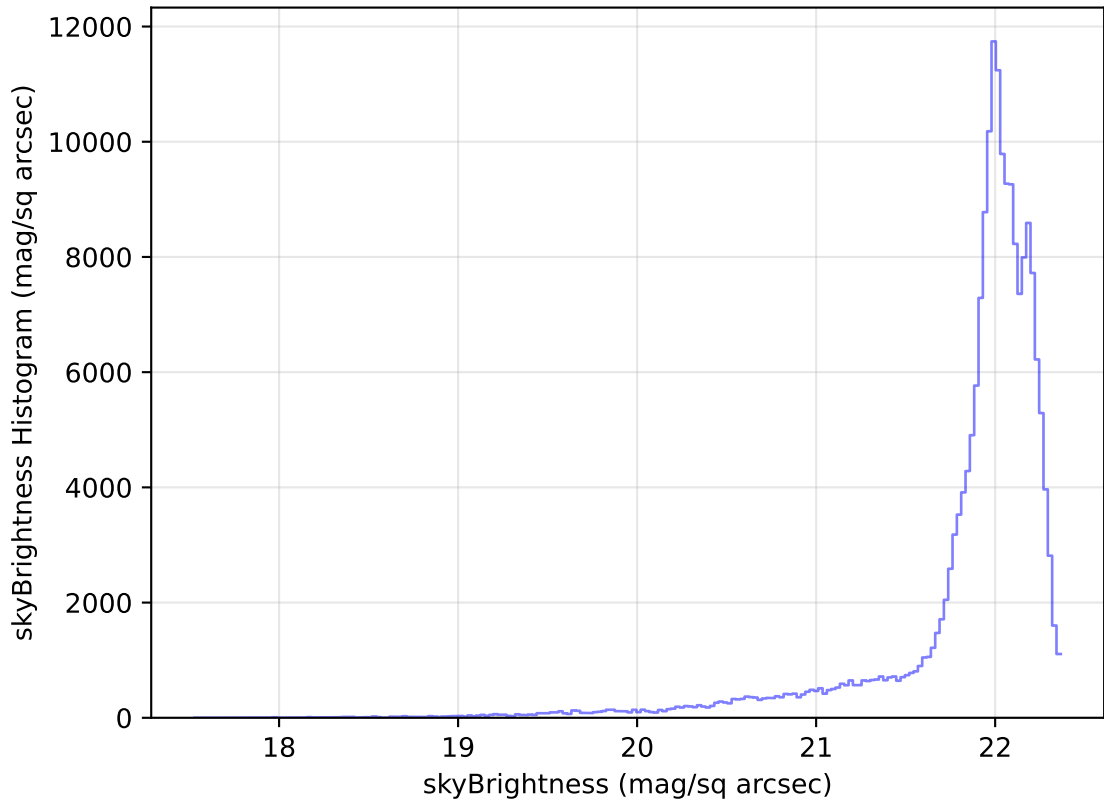
weather_cloudso36v3.4_10yrs All sky g band: skyBrightness Histogram
