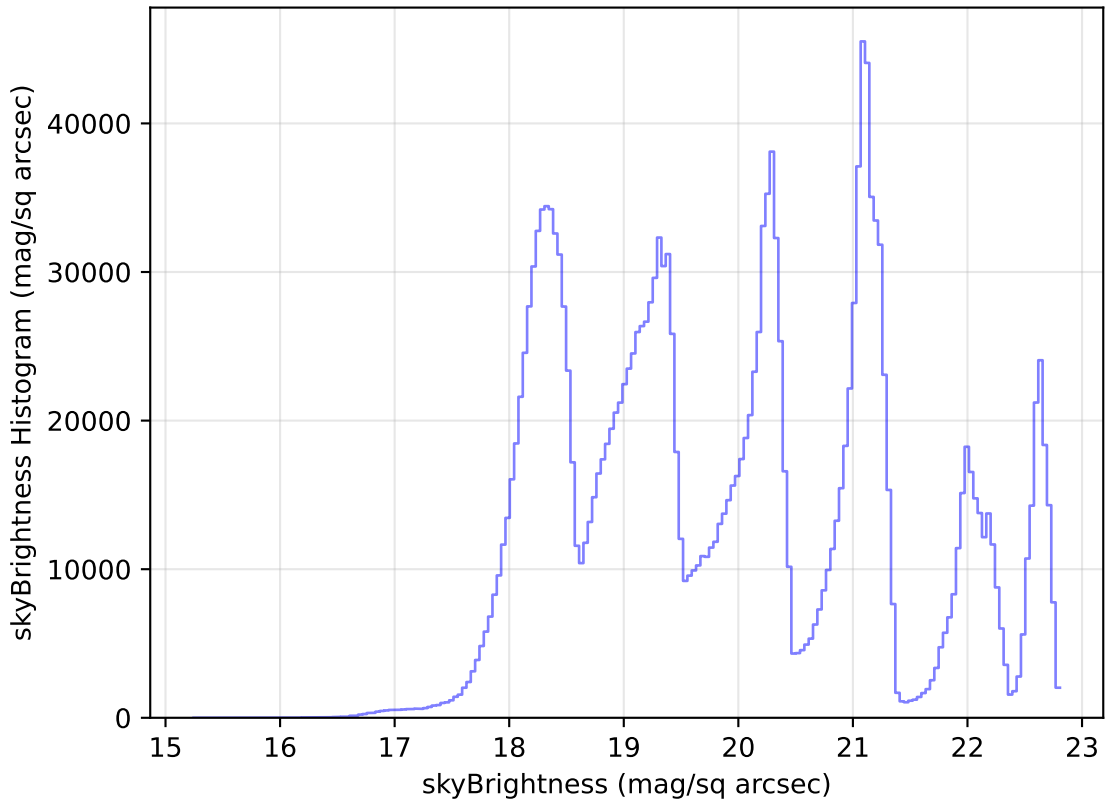
weather_cloudso36v3.4_10yrs All sky all bands: skyBrightness Histogram
