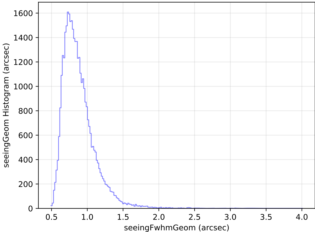
weather_cloudso36v3.4_10yrs Yr 1 z band: seeingGeom Histogram
