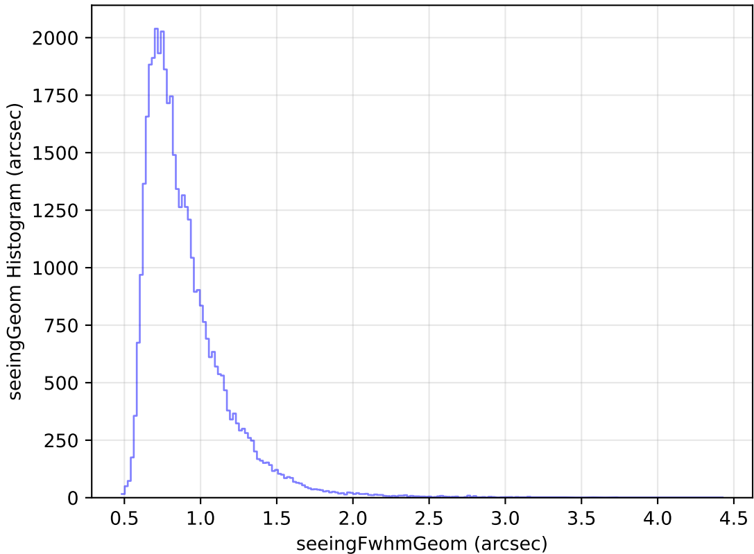
weather_cloudso36v3.4_10yrs Yr 1 r band: seeingGeom Histogram
