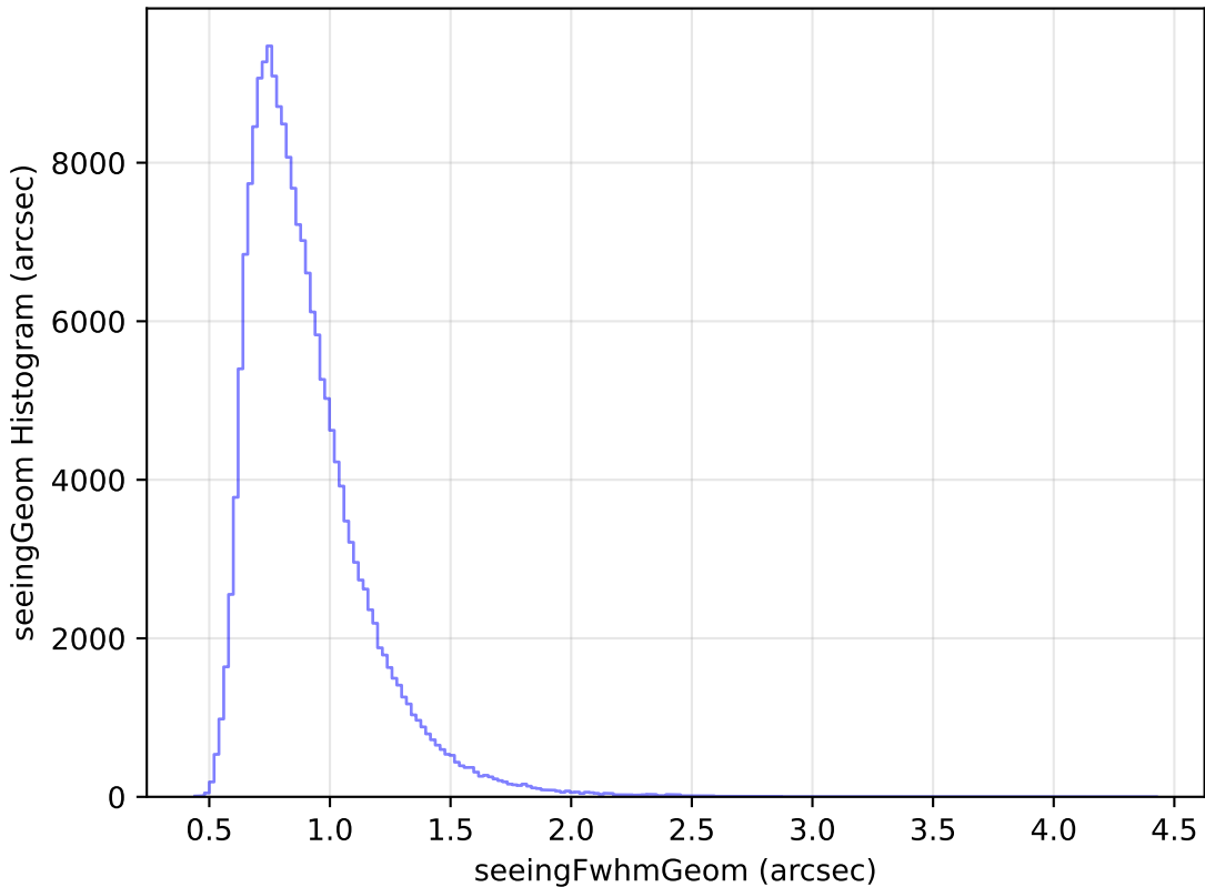
weather_cloudso36v3.4_10yrs Yr 1 all bands: seeingGeom Histogram
