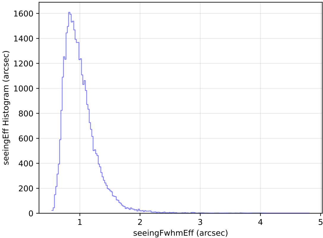
weather_cloudso36v3.4_10yrs Yr 1 z band: seeingEff Histogram
