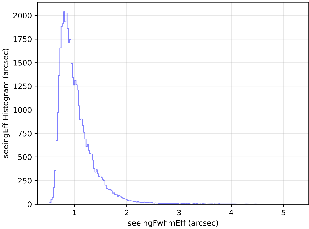
weather_cloudso36v3.4_10yrs Yr 1 r band: seeingEff Histogram
