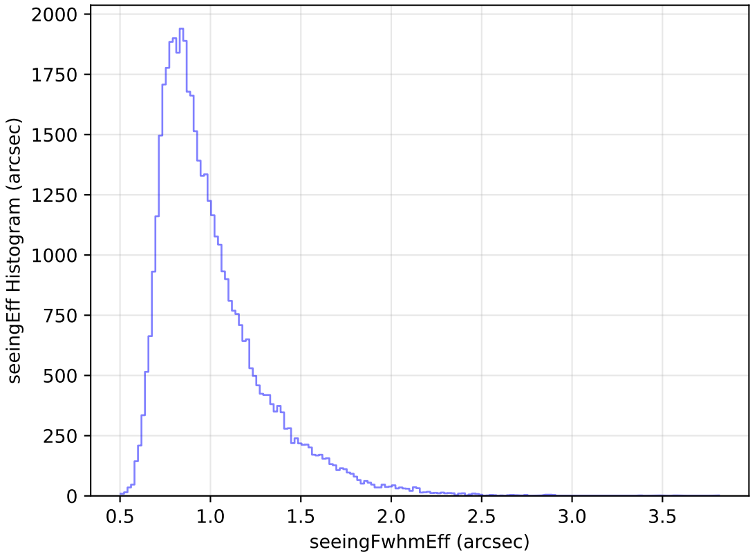
weather_cloudso36v3.4_10yrs Yr 1 i band: seeingEff Histogram
