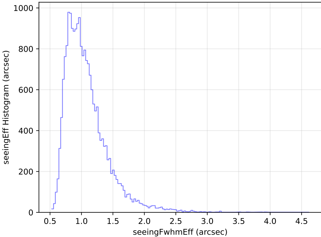
weather_cloudso36v3.4_10yrs Yr 1 g band: seeingEff Histogram
