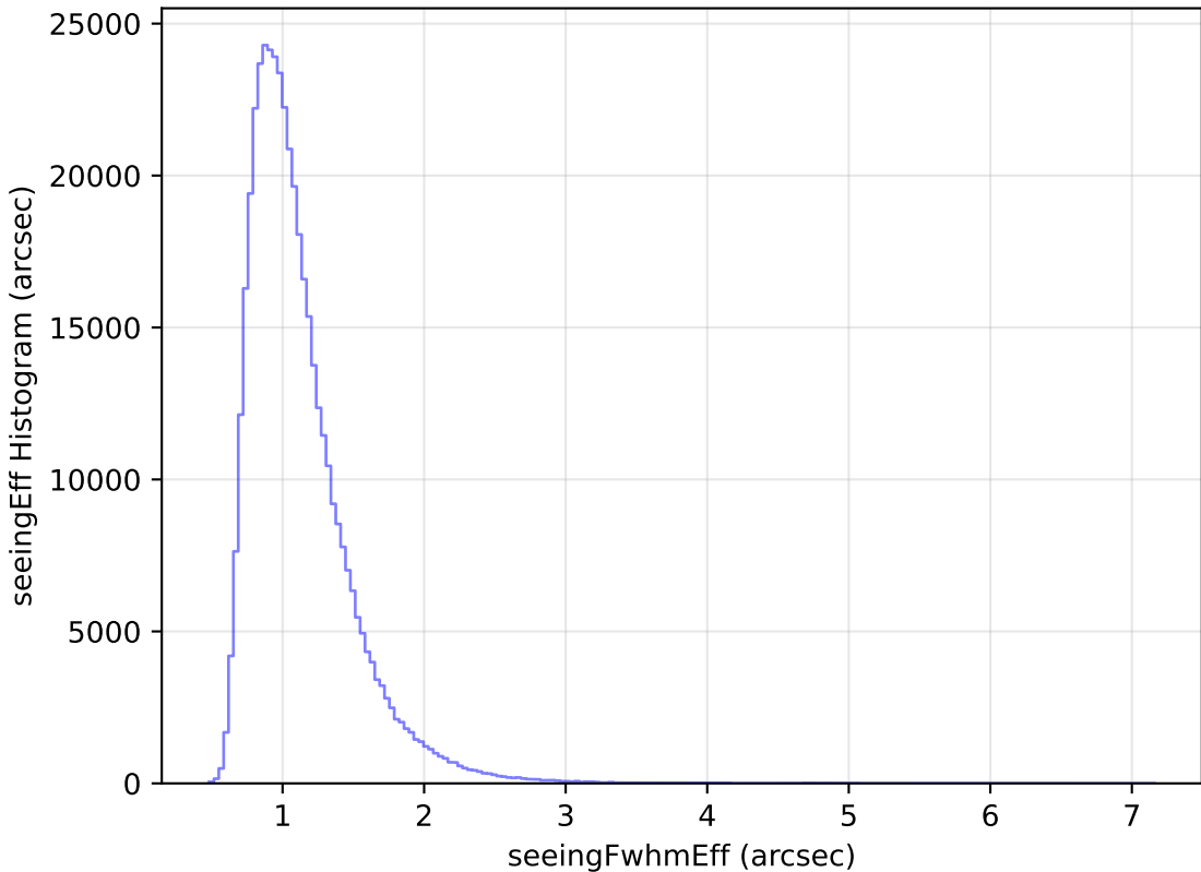
weather_cloudso36v3.4_10yrs WFD z band: seeingEff Histogram
