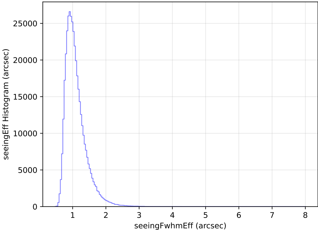
weather_cloudso36v3.4_10yrs WFD y band: seeingEff Histogram
