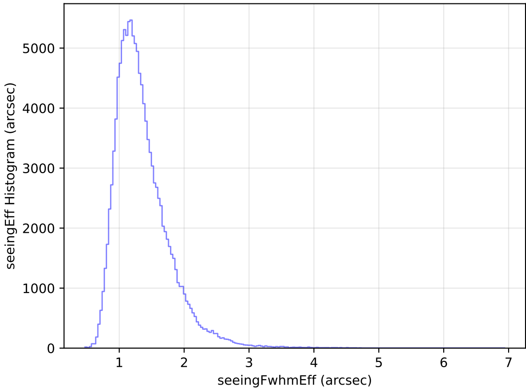
weather_cloudso36v3.4_10yrs WFD u band: seeingEff Histogram
