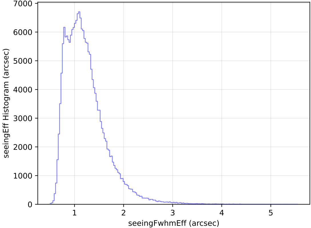
weather_cloudso36v3.4_10yrs WFD g band: seeingEff Histogram
