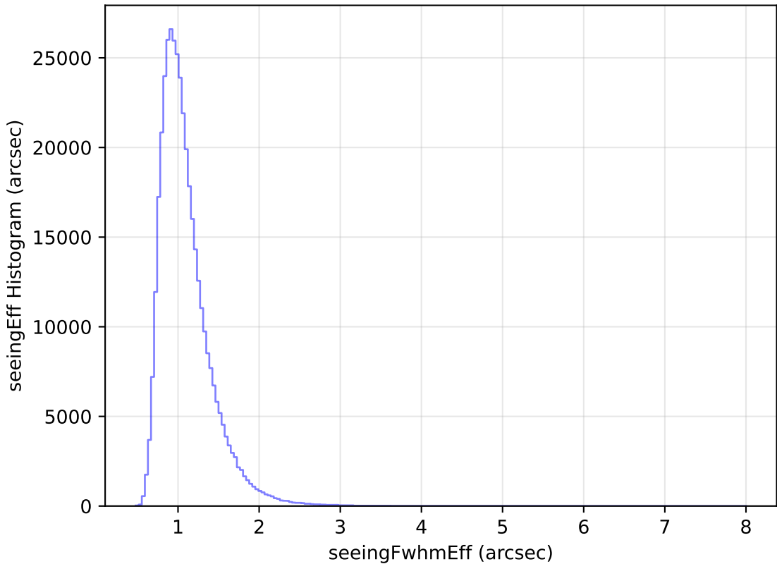
weather_cloudso36v3.4_10yrs All sky y band: seeingEff Histogram
