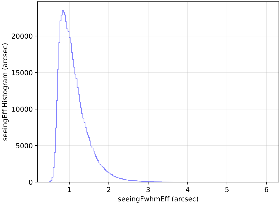
weather_cloudso36v3.4_10yrs All sky i band: seeingEff Histogram
