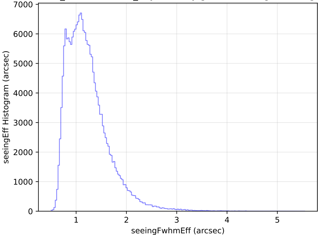
weather_cloudso36v3.4_10yrs All sky g band: seeingEff Histogram
