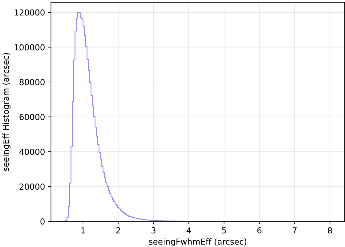
weather_cloudso36v3.4_10yrs All sky all bands: seeingEff Histogram
