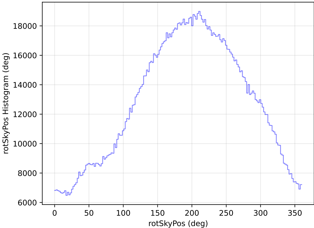
weather_cloudso36v3.4_10yrs WFD all bands: rotSkyPos Histogram
